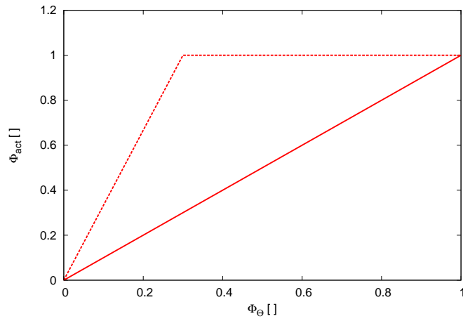
Figure B.11.: Metabolic activity \Phi_{\text{act}} as a function of water saturation \Phi_{\Theta} . The dashed line corresponds to x_{\Phi_{\Theta}, \text{sat}} = 0.3 and the solid line corresponds to x_{\Phi_{\Theta}, \text{sat}} = 1.0
