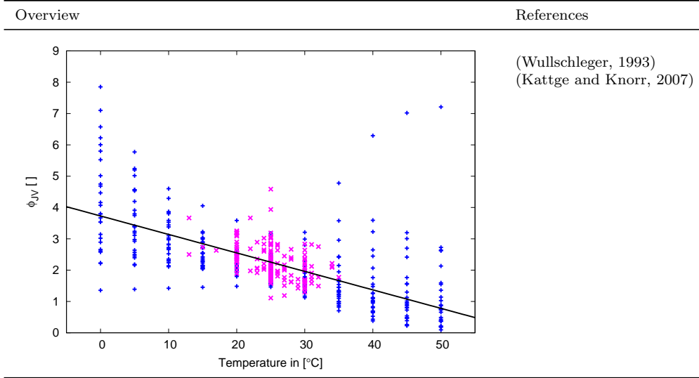
Figure B.13.: Ratio of J_{\text{max}} to V_{C,\text{max}} , \phi_{JV} , (black line) as a function of temperature. The magenta data points are taken from the study of Wullschlegel (1993) while the blue points are derived by the equations used in Kattge and Knorr (2007).
