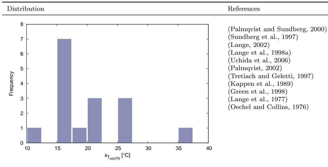
Figure B.9.: Overview of the distribution of the optimum temperature of photosynthesis x_{T_{\text{opt,PS}}} .
