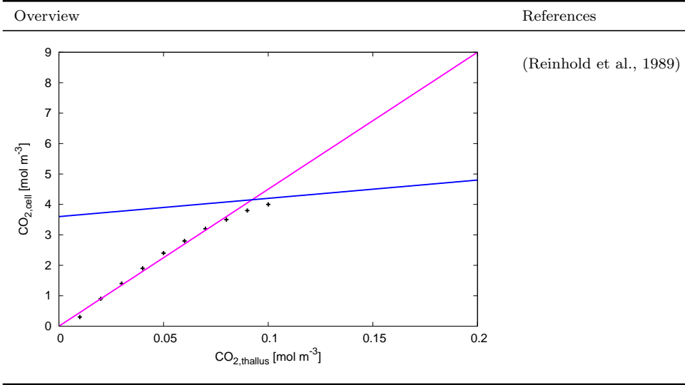
Figure B.14.: CO_2 concentration in the chloroplasts, CO_{2,cell} , as a function of pore space CO_2 concentration CO_{2,thallus} . The black data points are taken from the study of Reinhold et al. (1989). The minimum of the magenta and blue lines is used to fit the data.
